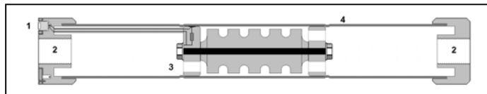
1 Meter 2 Pipe Connection 3 Zinc (Anode) 4 Copper Wall (Cathode)
